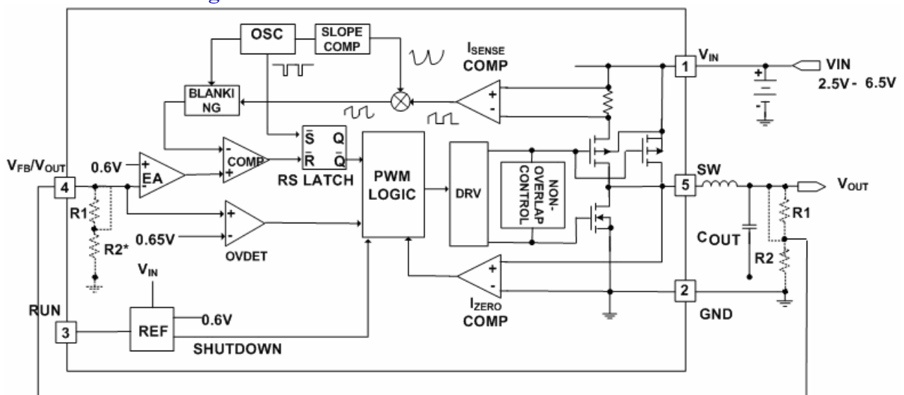
Figure 3. G2506 Block Diagram
