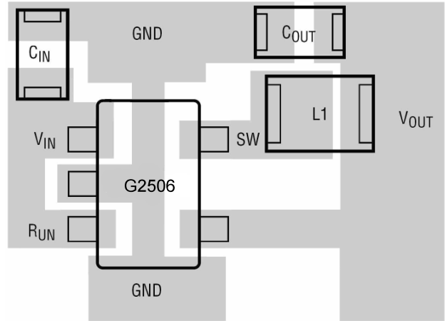
Figure5. G2506 Fixed output Suggested Layout
