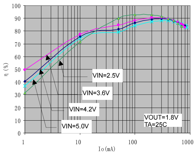
Figure 2. Typical Efficiency Curve
