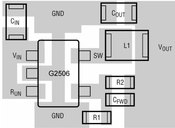
Figure4. G2506 ADJ output Suggested Layout
