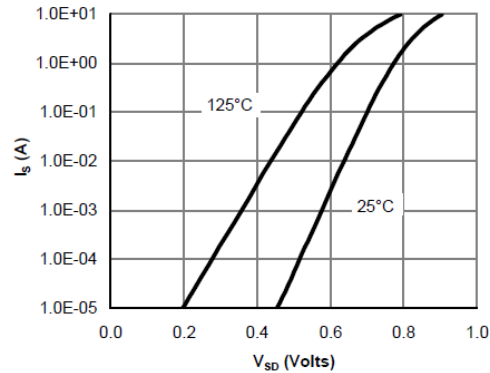
Figure 6: Body-Diode Characteristics
